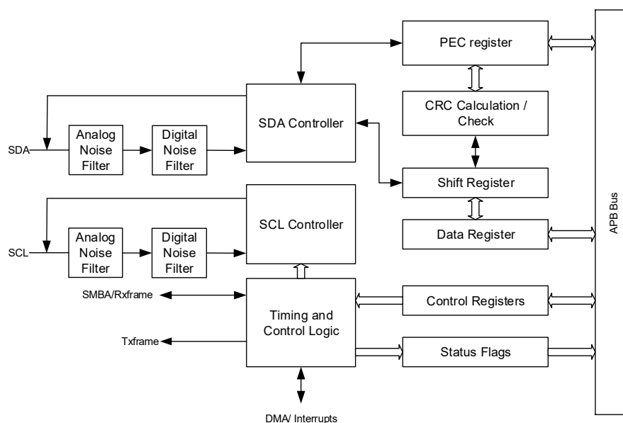
Figure 20-1. I2C module block diagram
