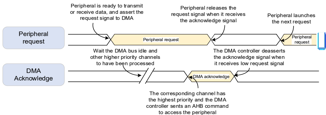
Figure 10-3. Handshake mechanism
