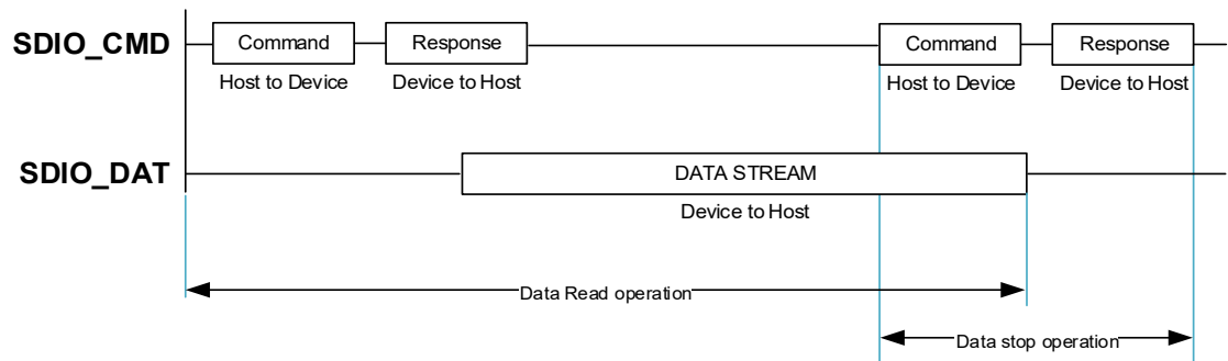
Figure 24-4. SDIO sequential read operation
