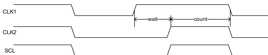
Figure 20-4. Clock synchronization
