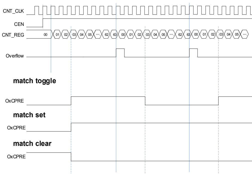
Figure 18-49. Output-compare under three modes
