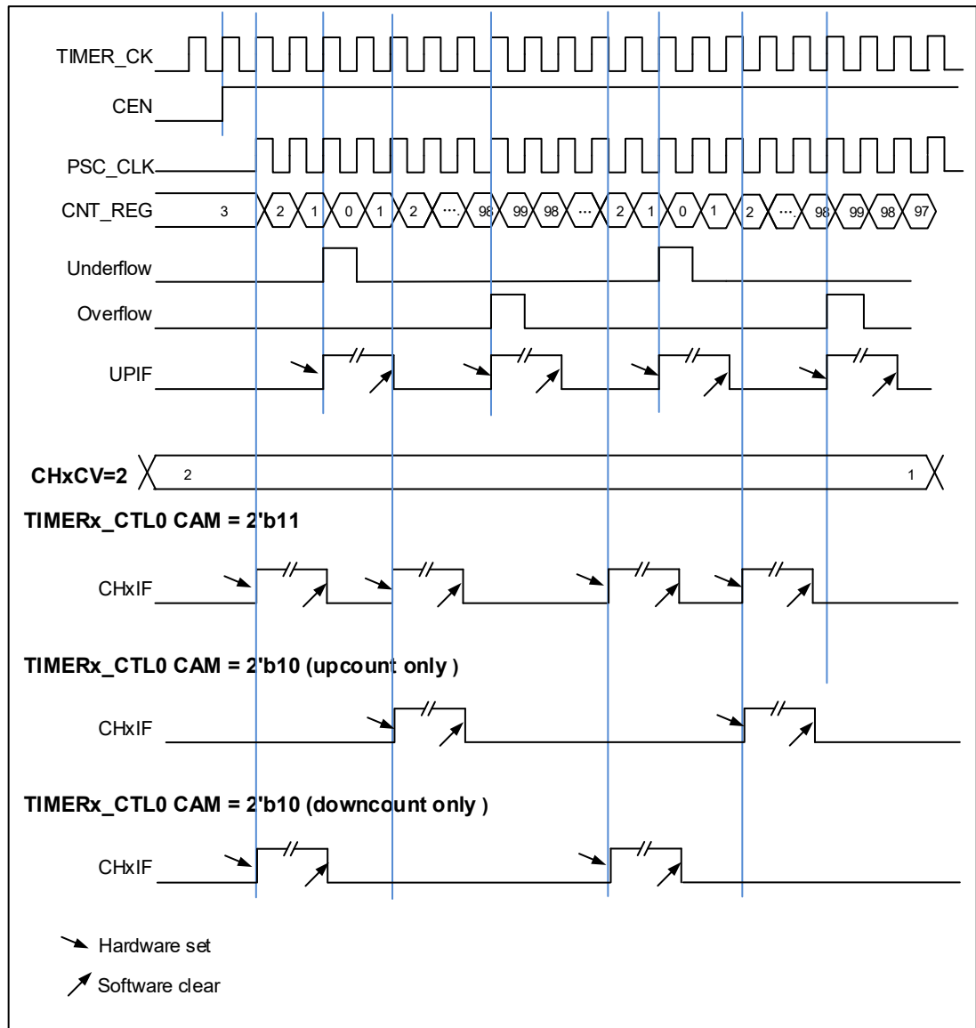
Figure 18-35. Timing chart of center-aligned counting mode
