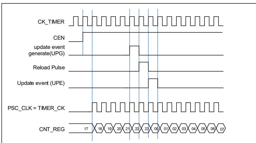
Figure 18-57. Timing chart of internal clock divided by 1
