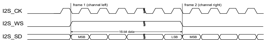
Figure 21-22. MSB justified standard timing diagram (DTLEN=00, CHLEN=0, CKPL=0)
