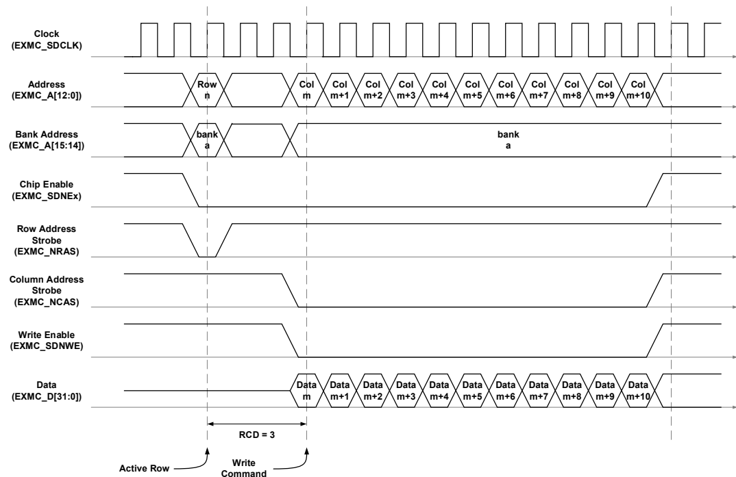
Figure 25-32. Burst write operation
