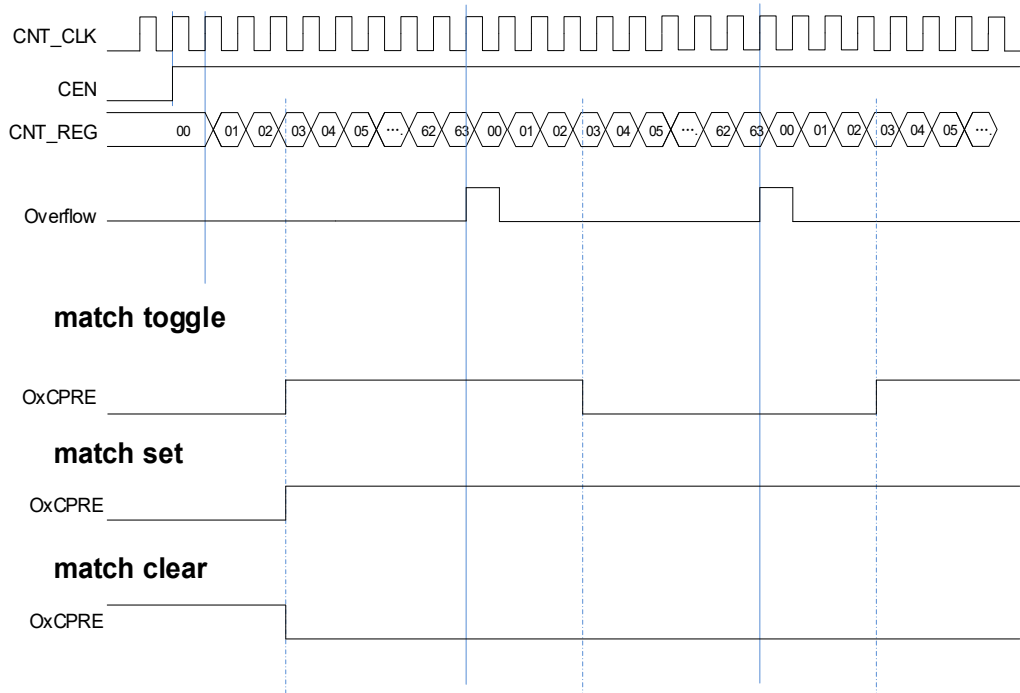
Figure 18-13. Output-compare under three modes
