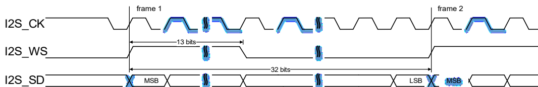
Figure 21-45. PCM standard long frame synchronization mode timing diagram (DTLEN=10, CHLEN=1, CKPL=1)
