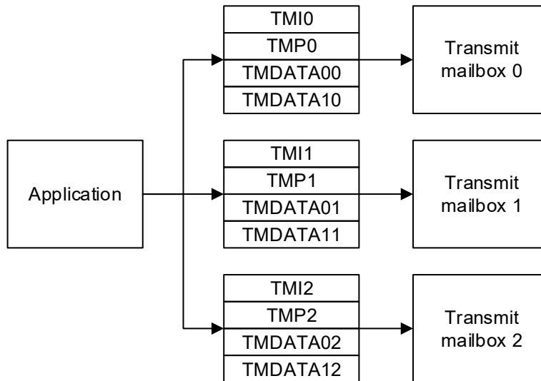
Figure 26-2. Transmission register
