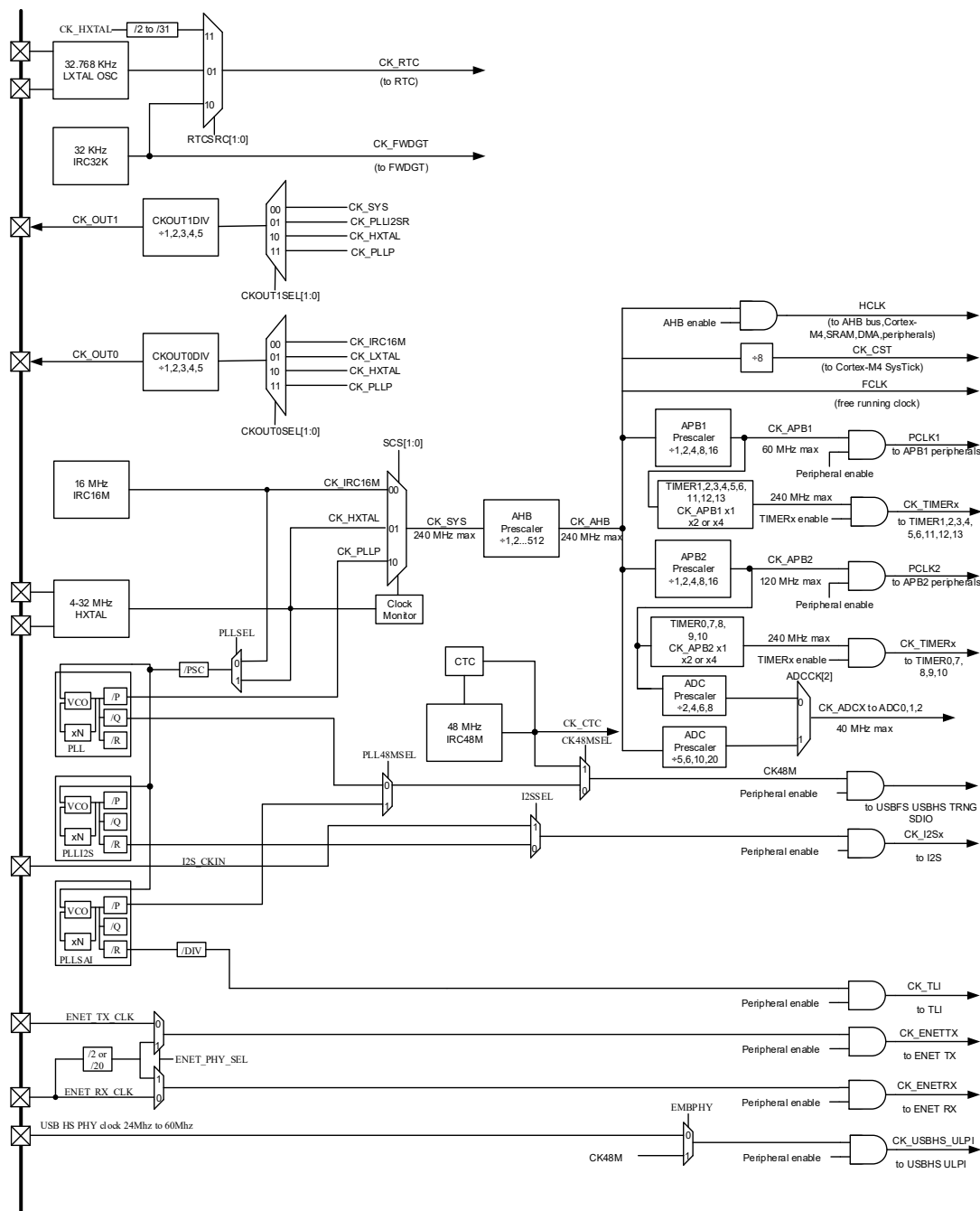
Figure 4-2. Clock tree
