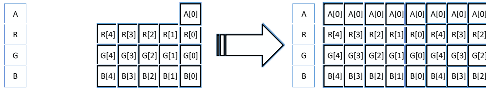
Figure 11-4. Pixel extension from 'ARGB1555' or 'ARGB4444' to 'ARGB8888'
