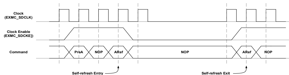
Figure 25-37. Process for self-refresh entry and exit
