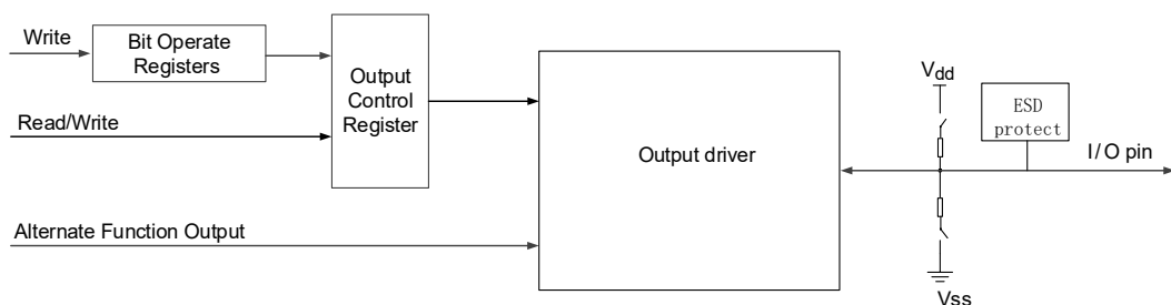
Figure 7-3. Basic structure of Output configuration
