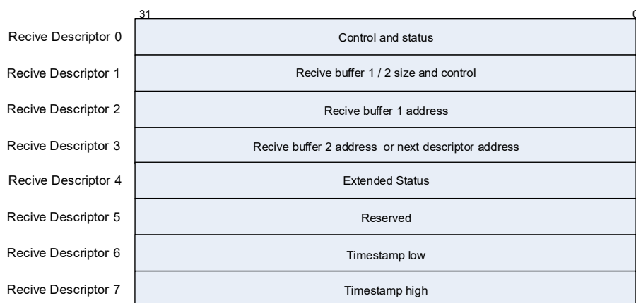
Figure 27-10. Receive descriptor in enhanced mode
