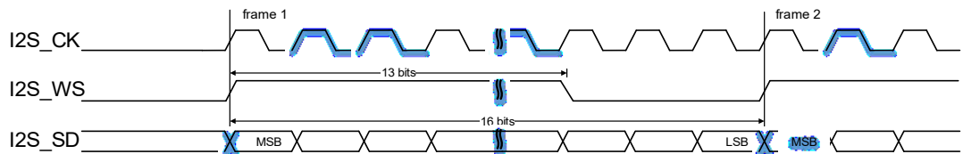
Figure 21-42. PCM standard long frame synchronization mode timing diagram (DTLEN=00, CHLEN=0, CKPL=0)
