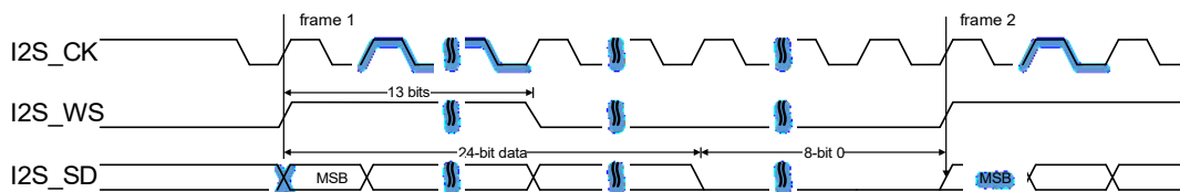
Figure 21-47. PCM standard long frame synchronization mode timing diagram (DTLEN=00, CHLEN=1, CKPL=0)
