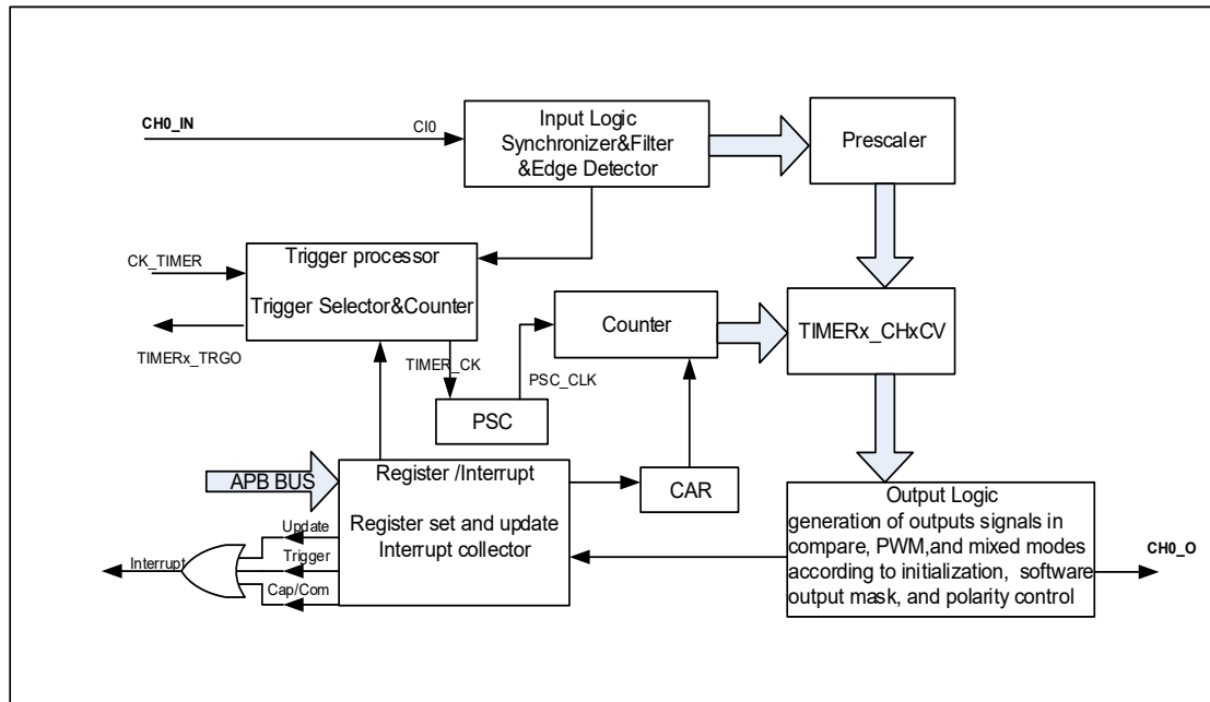
Figure 18-56. General level2 timer block diagram
