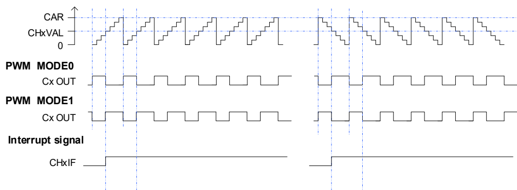
Figure 18-51. CAPWM timechart
