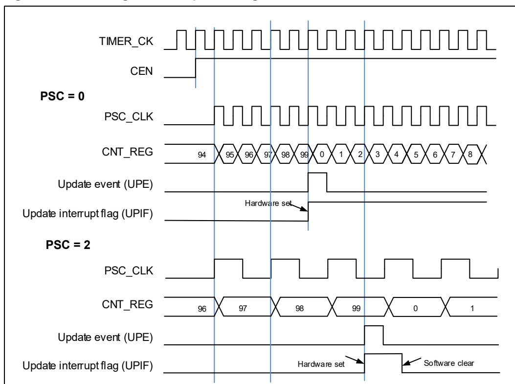
Figure 18-66. Timing chart of up counting mode, PSC=0/2
