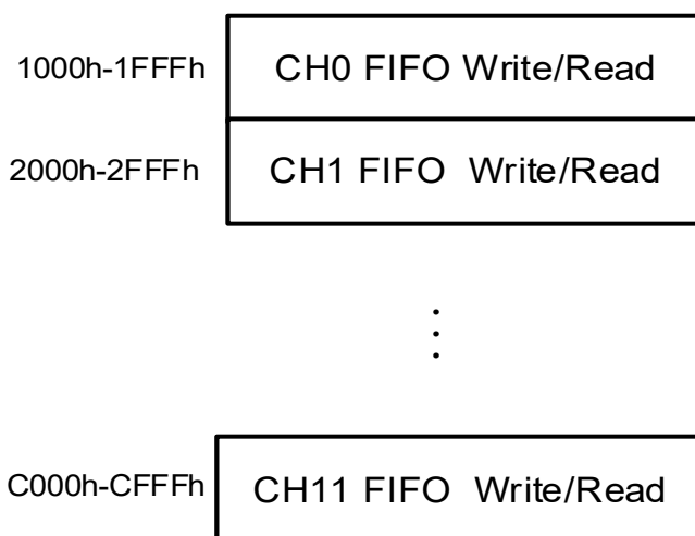
Figure 29-7. Host mode FIFO access register map
