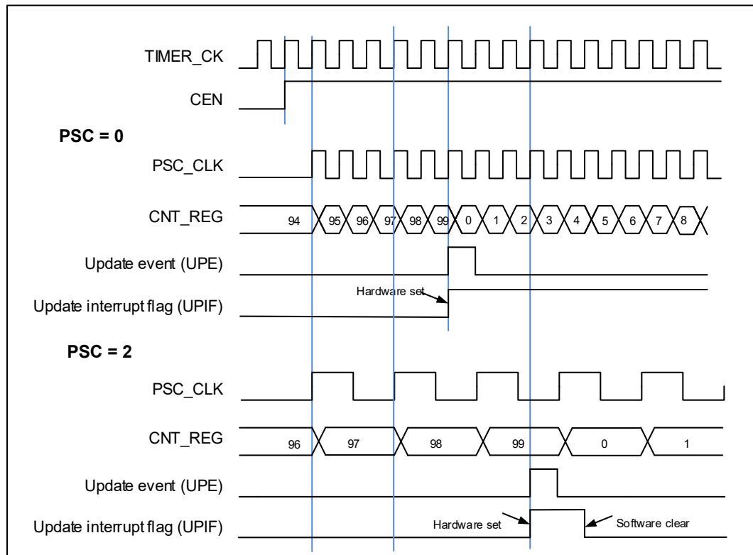
Figure 18-59. Timing chart of up counting mode, PSC=0/2
