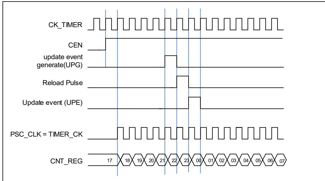
Figure 18-44. Timing chart of internal clock divided by 1
