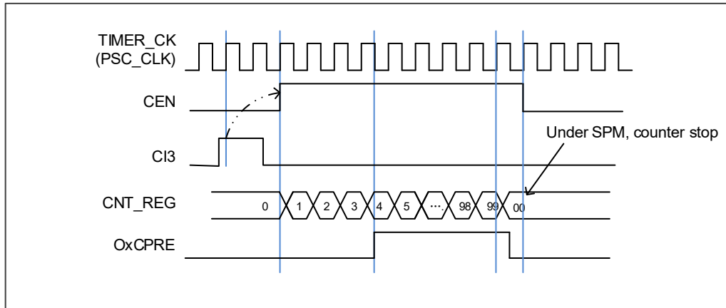
Figure 18-25. Single pulse mode, TIMERx\_CHxCV = 4 , TIMERx\_CAR = 99
