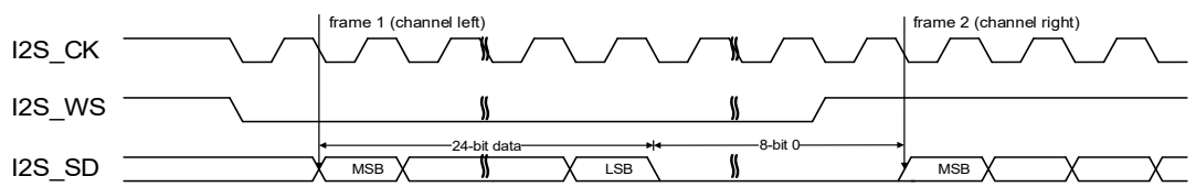
Figure 21-19. I2S Philips standard timing diagram (DTLEN=01, CHLEN=1, CKPL=1)
