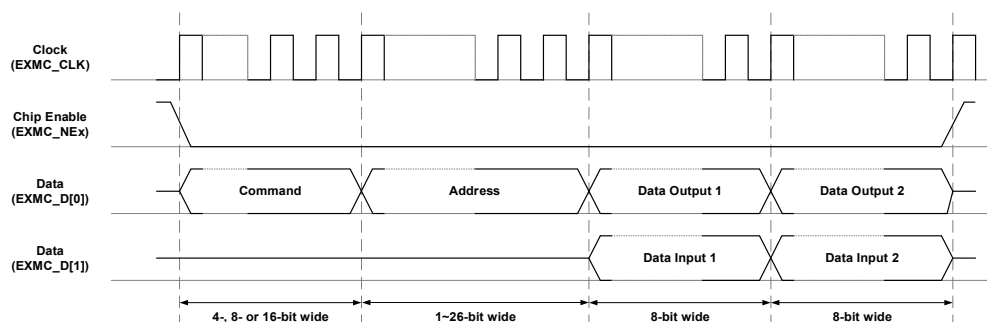
Figure 25-24. SPI-PSRAM access
