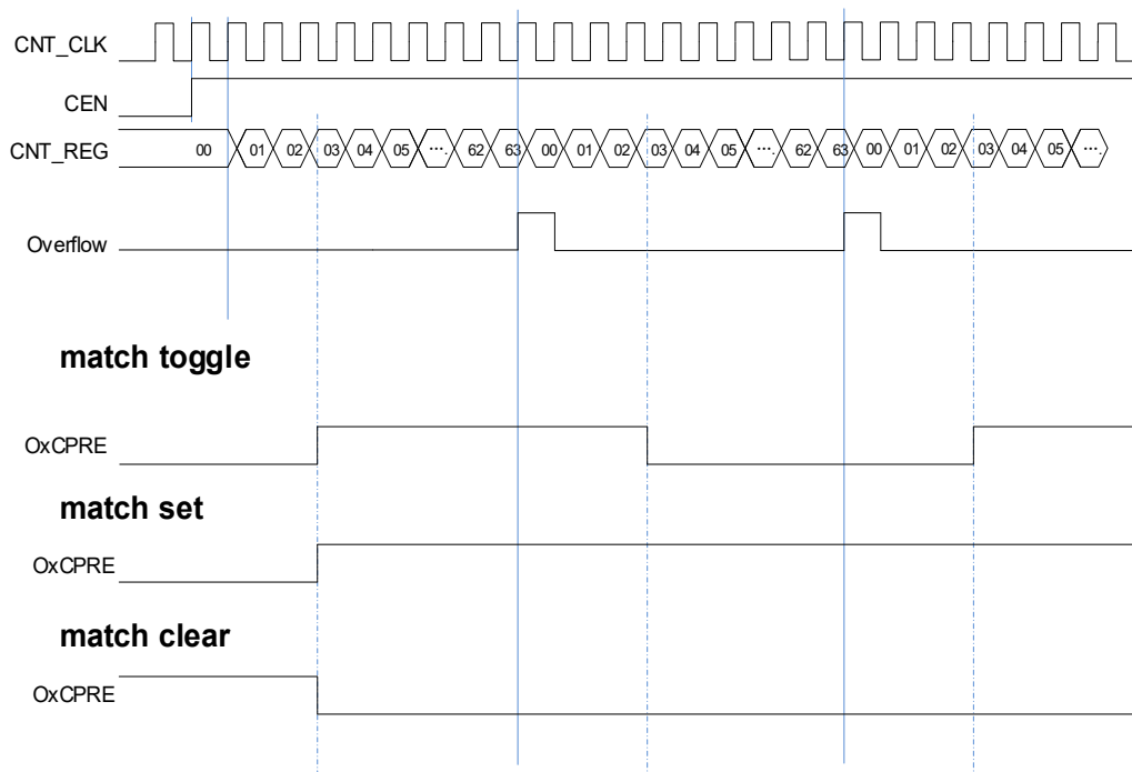
Figure 18-37. Output-compare under three modes
