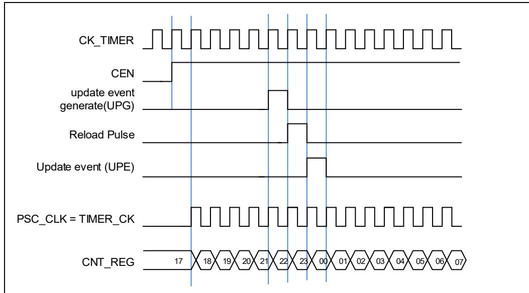
Figure 18-64. Timing chart of internal clock divided by 1
