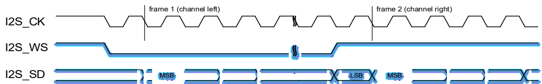
Figure 21-17. I2S Philips standard timing diagram (DTLEN=10, CHLEN=1, CKPL=1)
