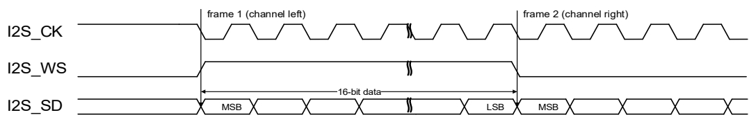
Figure 21-23. MSB justified standard timing diagram (DTLEN=00, CHLEN=0, CKPL=1)
