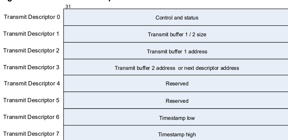
Figure 27-8. Transmit descriptor in enhanced mode
