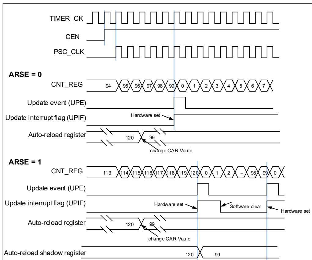
Figure 18-67. Up-counter timechart, change TIMERx_CAR on the go
