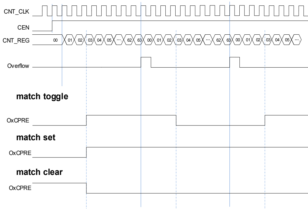
Figure 18-62. Output-compare under three modes
