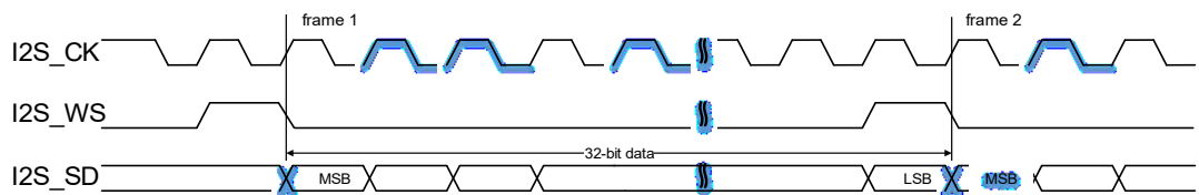
Figure 21-37. PCM standard short frame synchronization mode timing diagram (DTLEN=10, CHLEN=1, CKPL=1)
