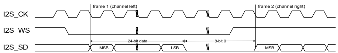
Figure 21-18. I2S Philips standard timing diagram (DTLEN=01, CHLEN=1, CKPL=0)
