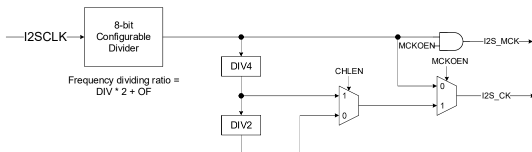
Figure 21-50. Block diagram of I2S clock generator
