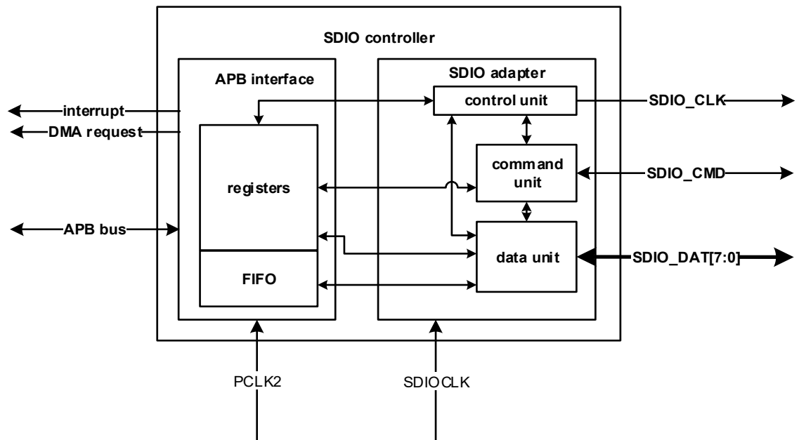
Figure 24-6. SDIO block diagram
