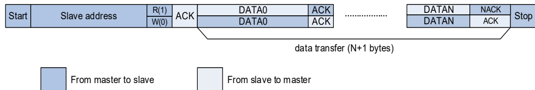
Figure 20-7. I2C communication flow with 10-bit address (Master Transmit)
