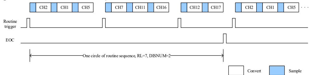
Figure 14-6. Discontinuous operation mode
