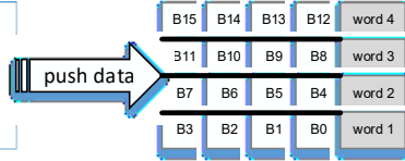
Figure 10-4. Data packing/unpacking when PWIDTH = '00'
