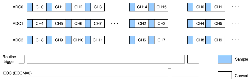
Figure 14-14. Routine parallel mode on 16 channels
