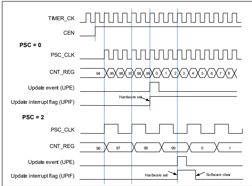
Figure 18-31. Timing chart of up counting mode, PSC=0/2
