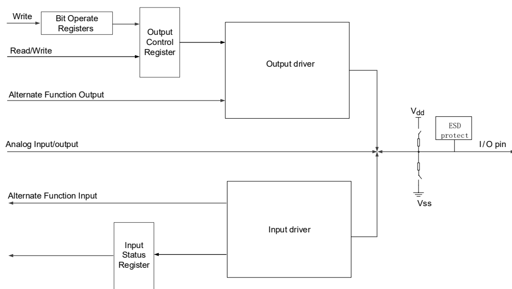
Figure 7-1. Basic structure of a standard I / O
