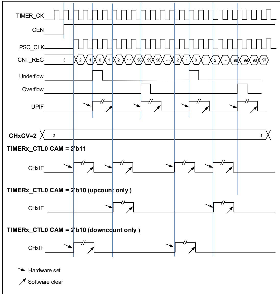
Figure 18-8. Center-aligned counter timechart
