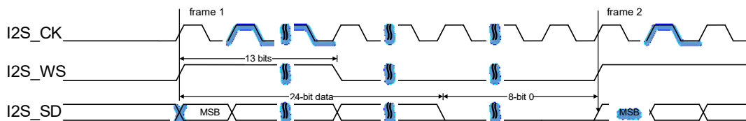
Figure 21-46. PCM standard long frame synchronization mode timing diagram (DTLEN=01, CHLEN=1, CKPL=1)
